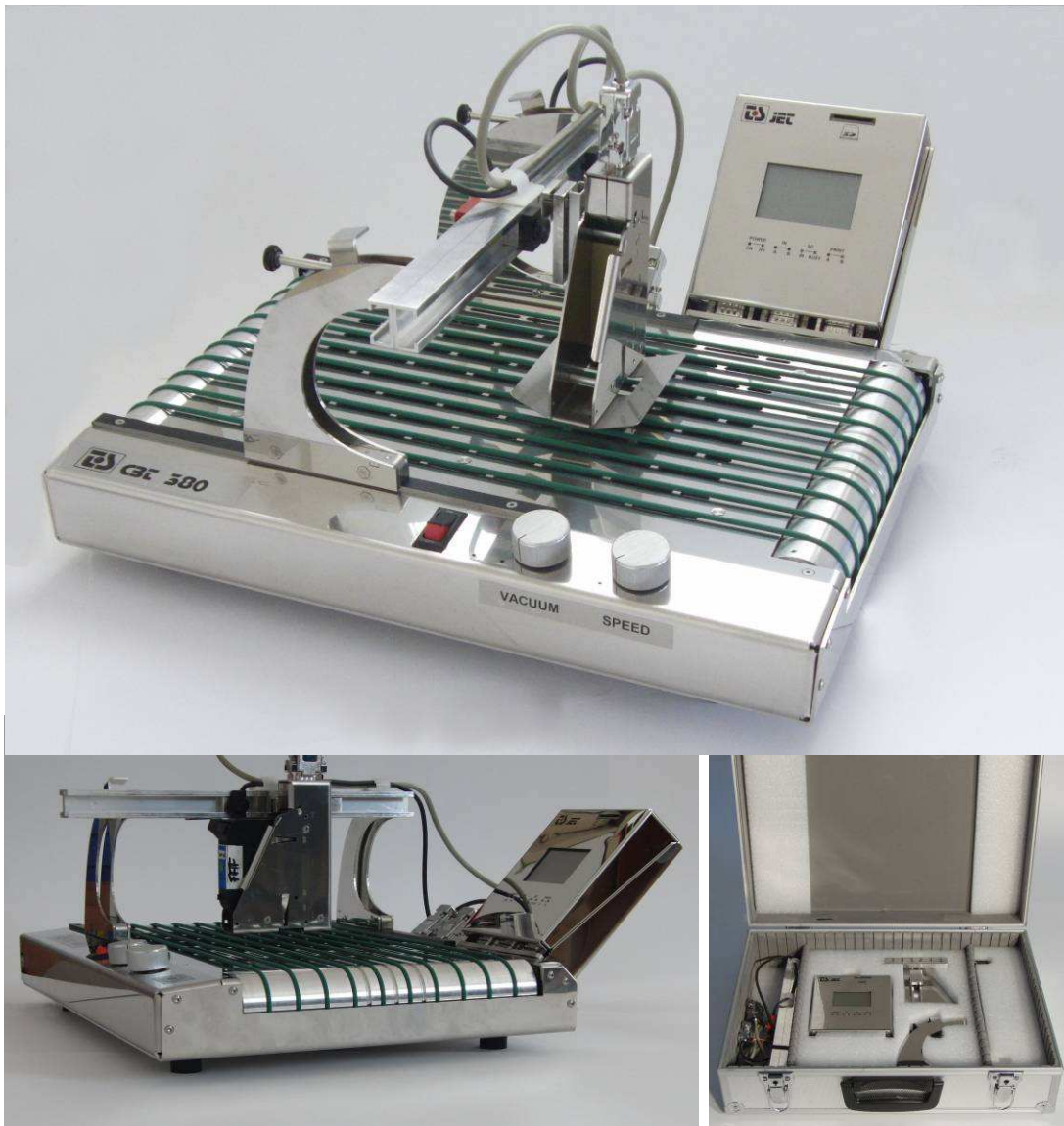
Mobile conveyor for advertising print applications CBT380
